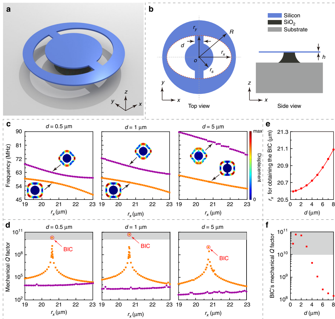
Fig. 2 Design and numerical simulation of mechanical BIC in a micromechanical resonator. a Illustration of the wheel-shaped micromechanical resonator that supports mechanical BIC. b Top and side views of the micromechanical resonator, with dimension labels. c Simulated frequencies of modes A' and B' of the micromechanical resonator as a function of r_x for d = 0.5 , 1 , and 5 \mu\text{m} . The insets show the corresponding modal displacement profiles. d Simulated mechanical Q factors of modes A' and B' as a function of r_x for d = 0.5 , 1 , and 5 \mu\text{m} . The BIC point where the highest mechanical Q factor is achieved is marked in each plot. e The value of r_x for obtaining the BIC as a function of d . f Simulated mechanical Q factor of the BIC as a function of d . In (c–f), the fixed geometric parameters of the micromechanical resonator are r_y = 18.7 \mu\text{m} , R = 26.1 \mu\text{m} , r_s = 14.7 \mu\text{m} , and h = 220 nm. In (d) and (f), the gray areas indicate the regimes reaching the limit of numerical simulation, where the simulated results do not converge
